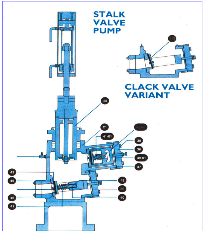
Latham Vertical Ram Pump
