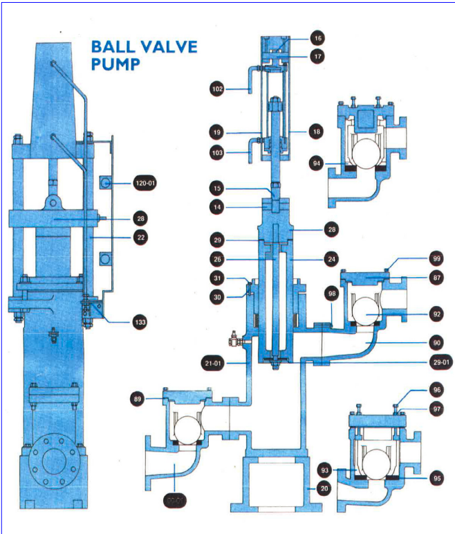
WILLET PUMPS TYPES
