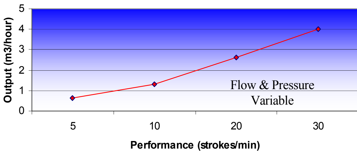
Output For 110mm Pump
