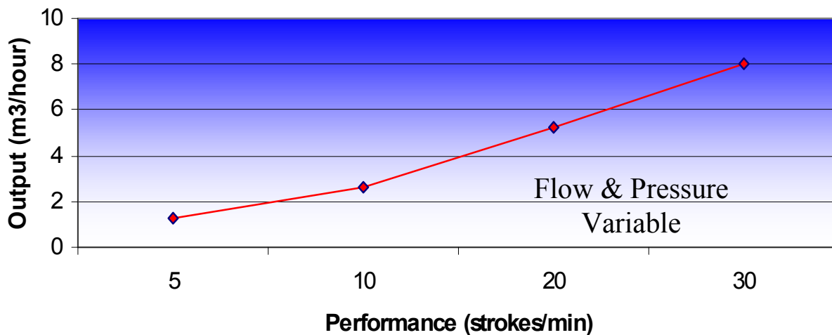
Output For 160mm Pump
